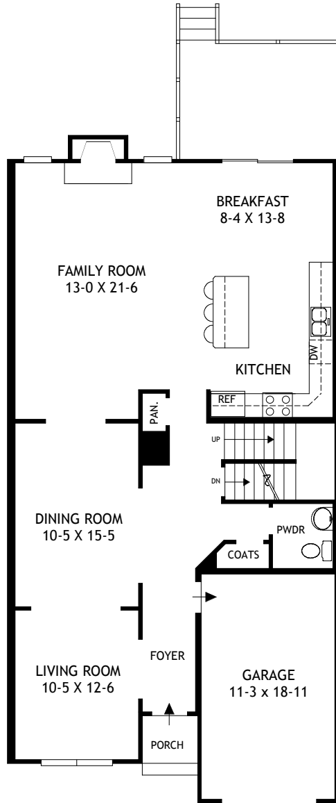
FIRST FLOOR
